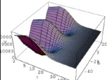
Kahler modulus potential T=\tau+i\theta
